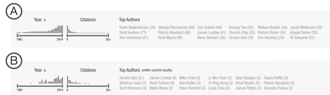
Fig. 4. (A) Histogram filters and Author List for all papers in the CHI and UIST corpus and (B) after searching for the term “tangible”.
