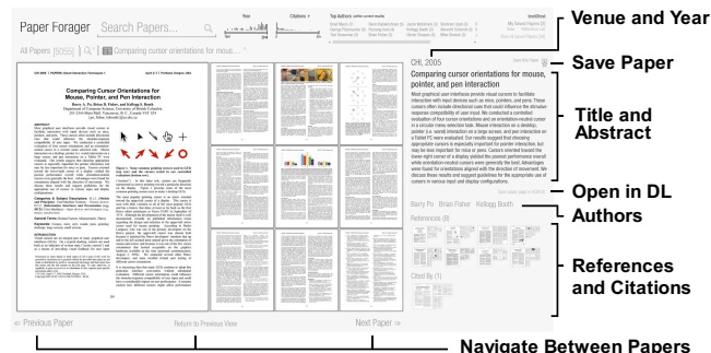
Fig. 10. Interface elements of the single paper view.
