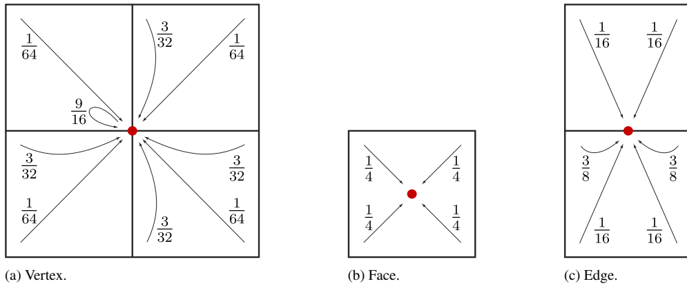
Fig. 6. Subdivision stencils for the Catmull–Clark scheme. Each of the stencils are used for computing the coordinates of vertices of the type indicated by red dot.
