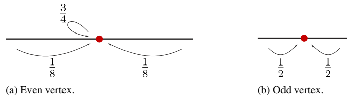
Fig. 5. Subdivision stencils for cubic b-splines.
