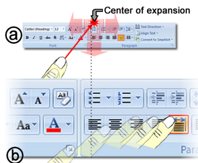
Figure 1 - TouchZoom. (a) The ribbon expands at the intersection of a finger's motion vector and the top edge of the ribbon. (b) After the expansion, finger movement is adjusted to acquire the new position of the highlighted goal target icon.
