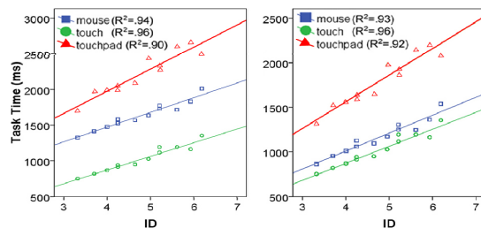
Figure 4 –Task completion time with homing time (left) and without homing time (right) by the index of difficulty.
