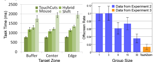
Figure 11 – Left: average task time shown for each target zone by technique. Right: off-screen rate shown by group sizes.
